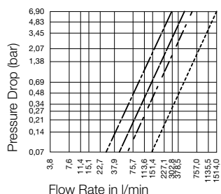
Flow Capacity with MIL-H-6083 Hydraulic Fluid at 32°C +/-1,5°C
