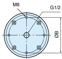
Ø150 mm (6") Aluminium end plate version
